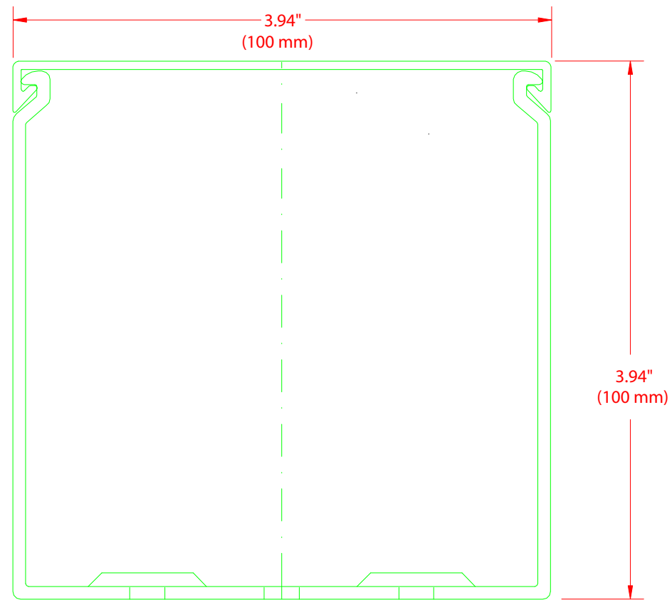
FRONT SECTION
