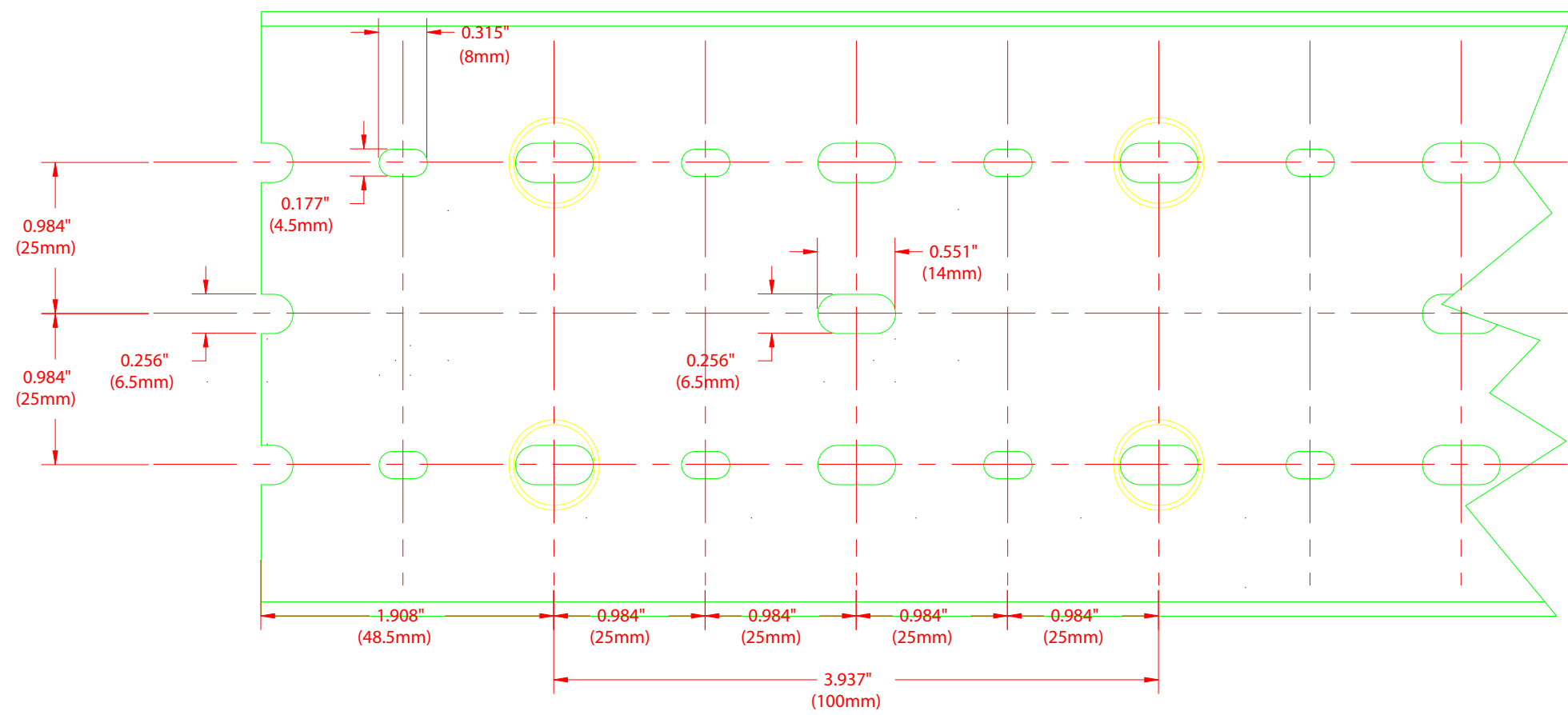
BASE PERFORATION
