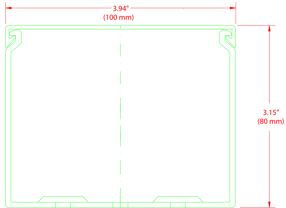
FRONT SECTION
