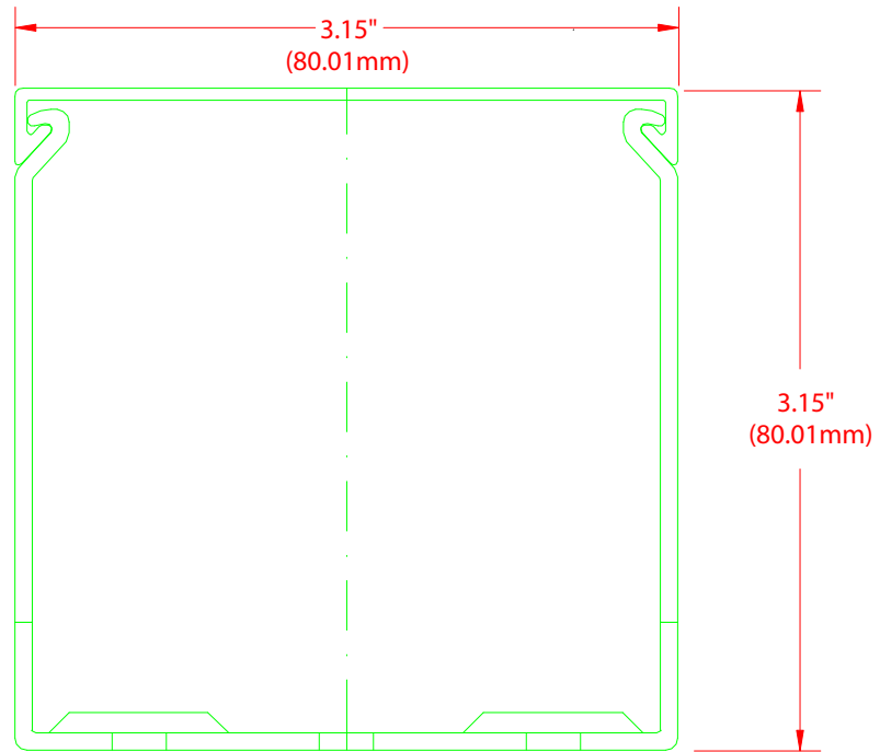
FRONT SECTION
