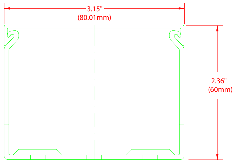
FRONT SECTION
