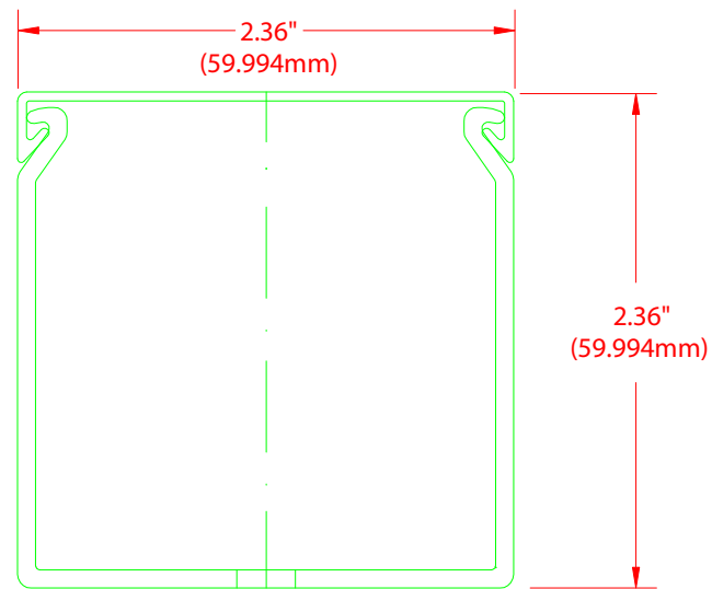
FRONT SECTION
