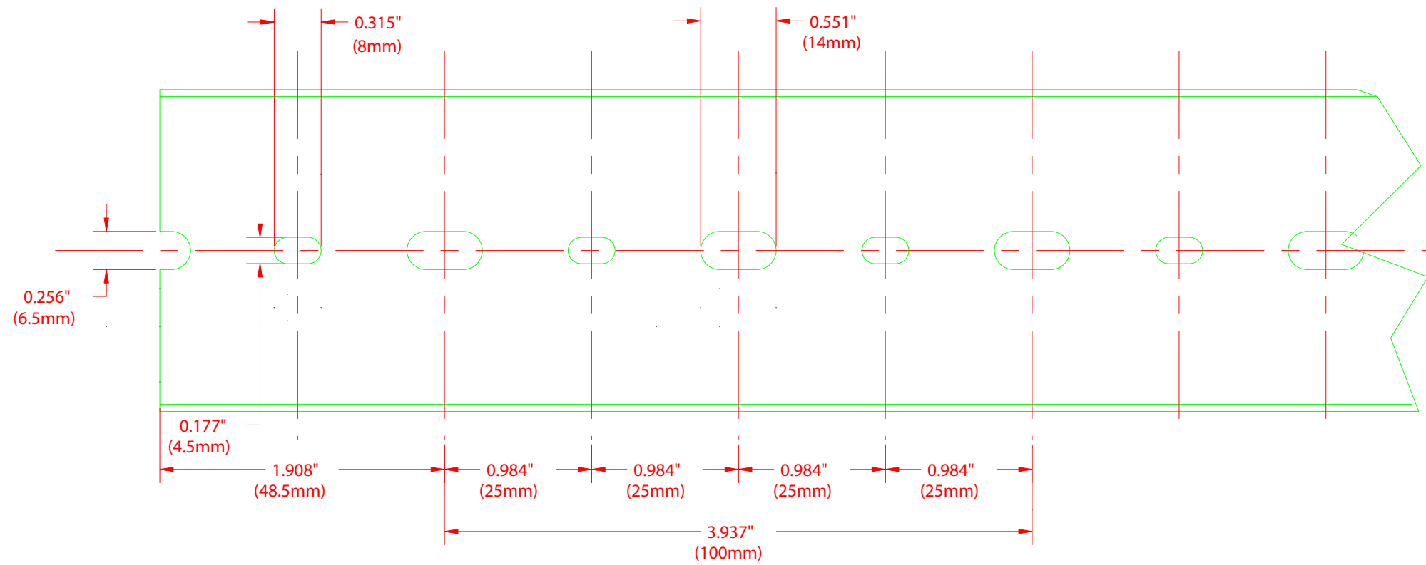
BASE PERFORATION
