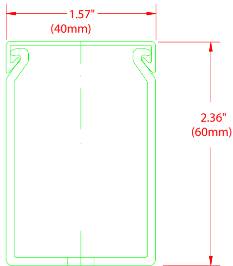
FRONT SECTION
