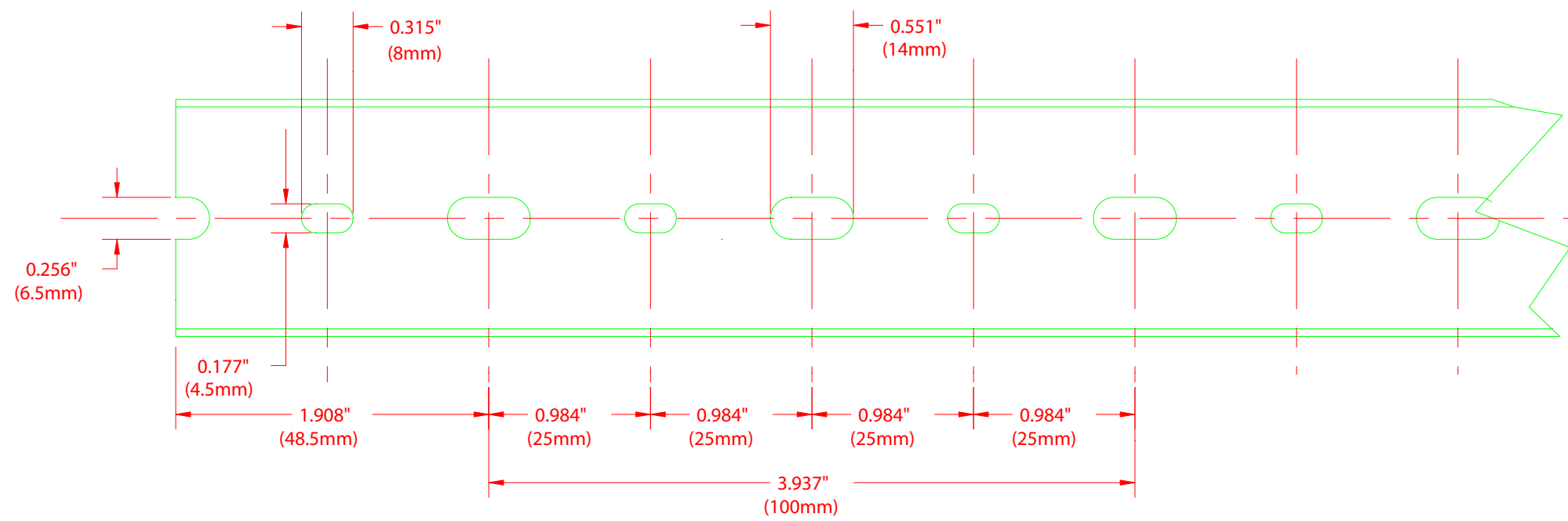
BASE PERFORATION
