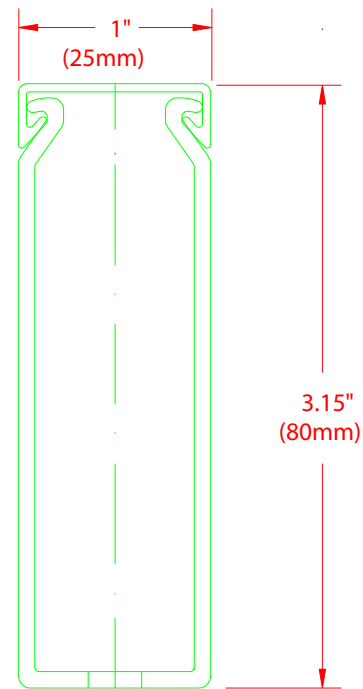
FRONT SECTION
