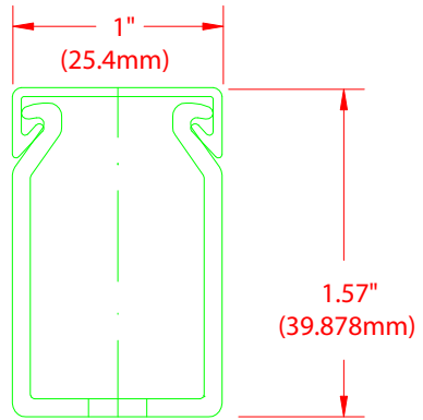
FRONT SECTION
