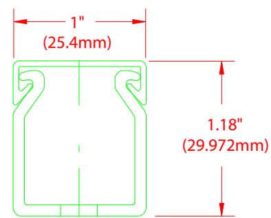
FRONT SECTION
