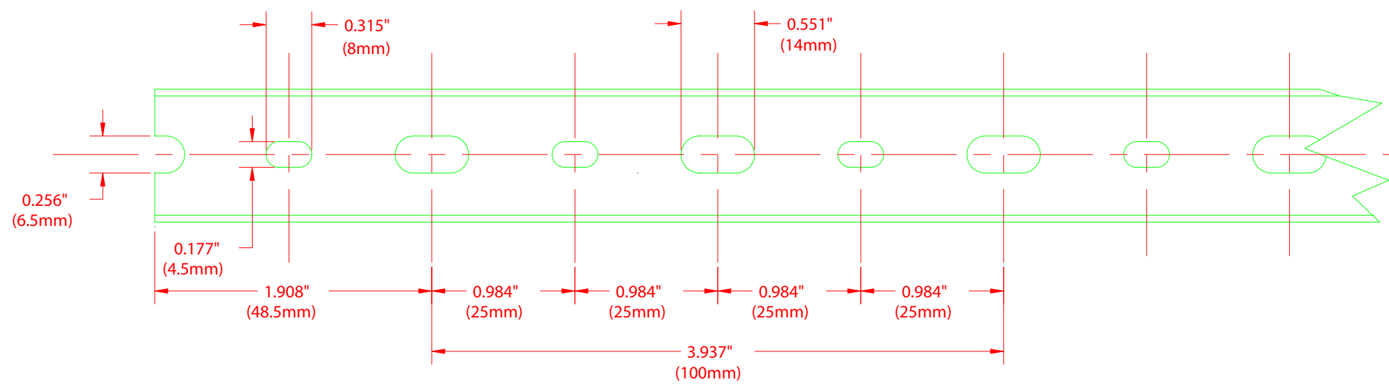
BASE PERFORATION
