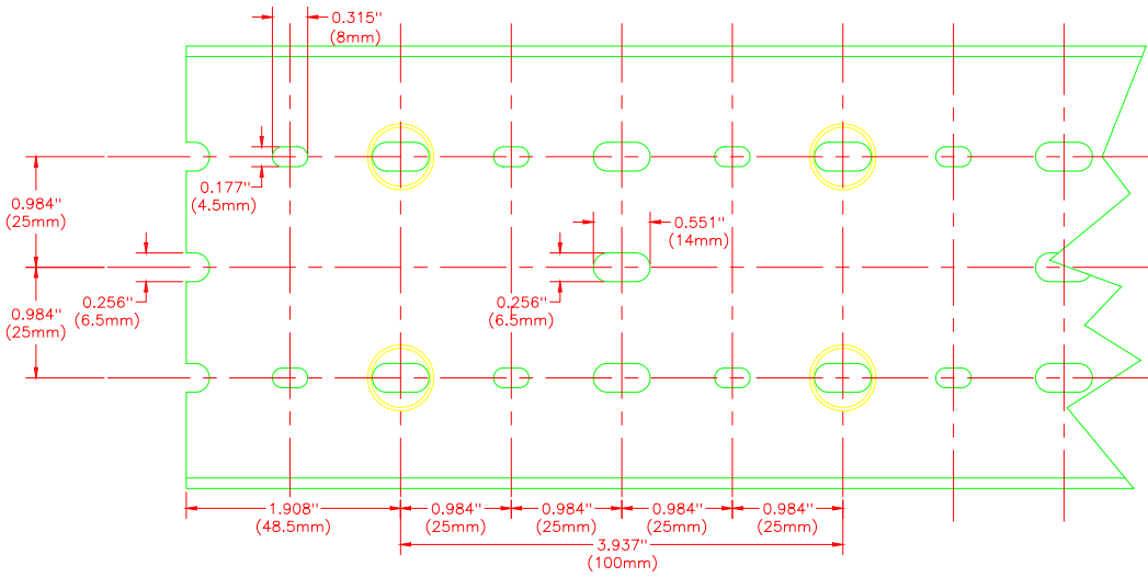
BASE PERFORATION
