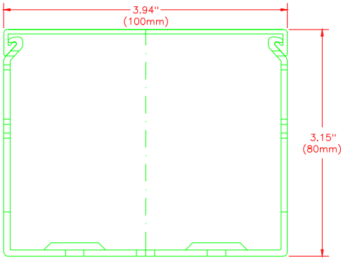
FRONT SECTION
