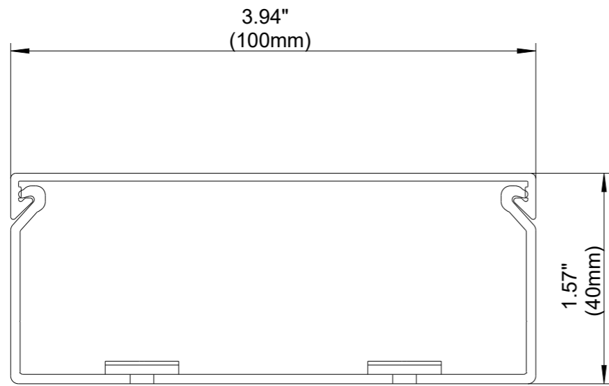
FRONT SECTION
