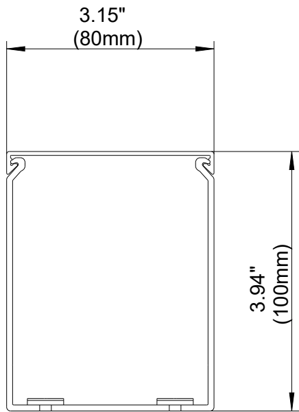
SCALE 1:2 FRONT SECTION
