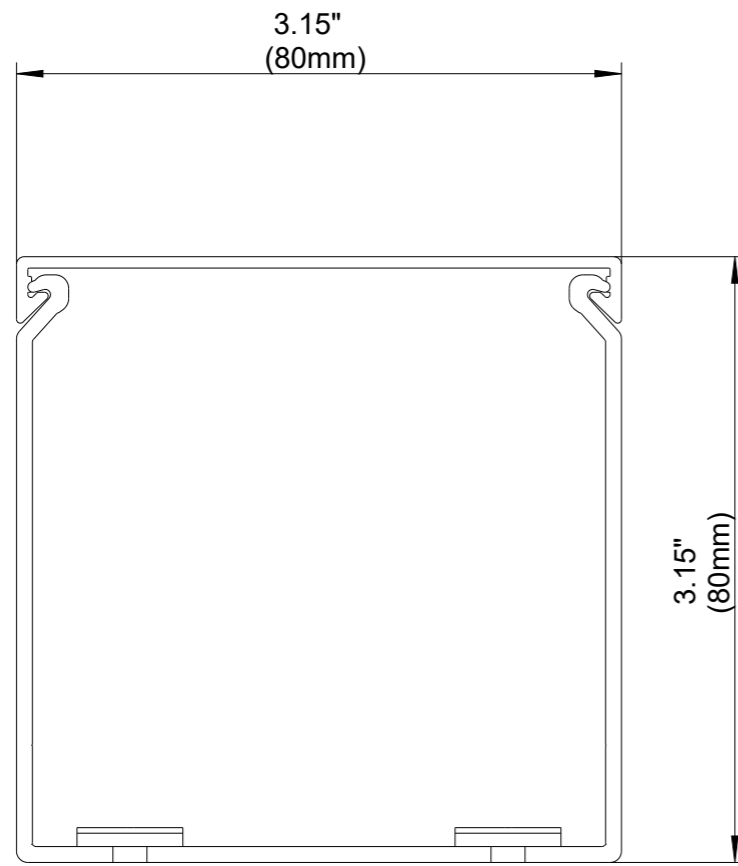
FRONT SECTION
