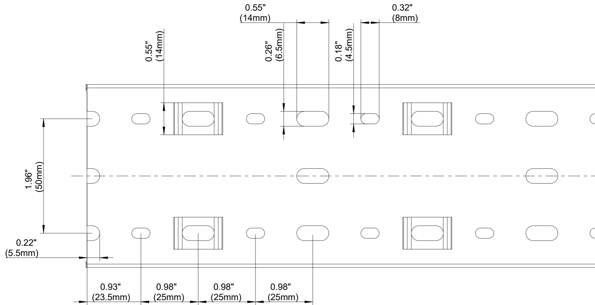
BASE PERFORATION
