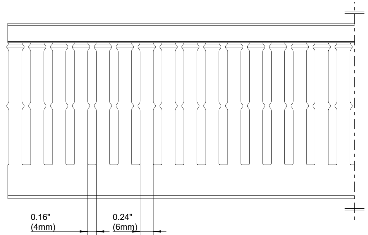
SIDE SECTION
