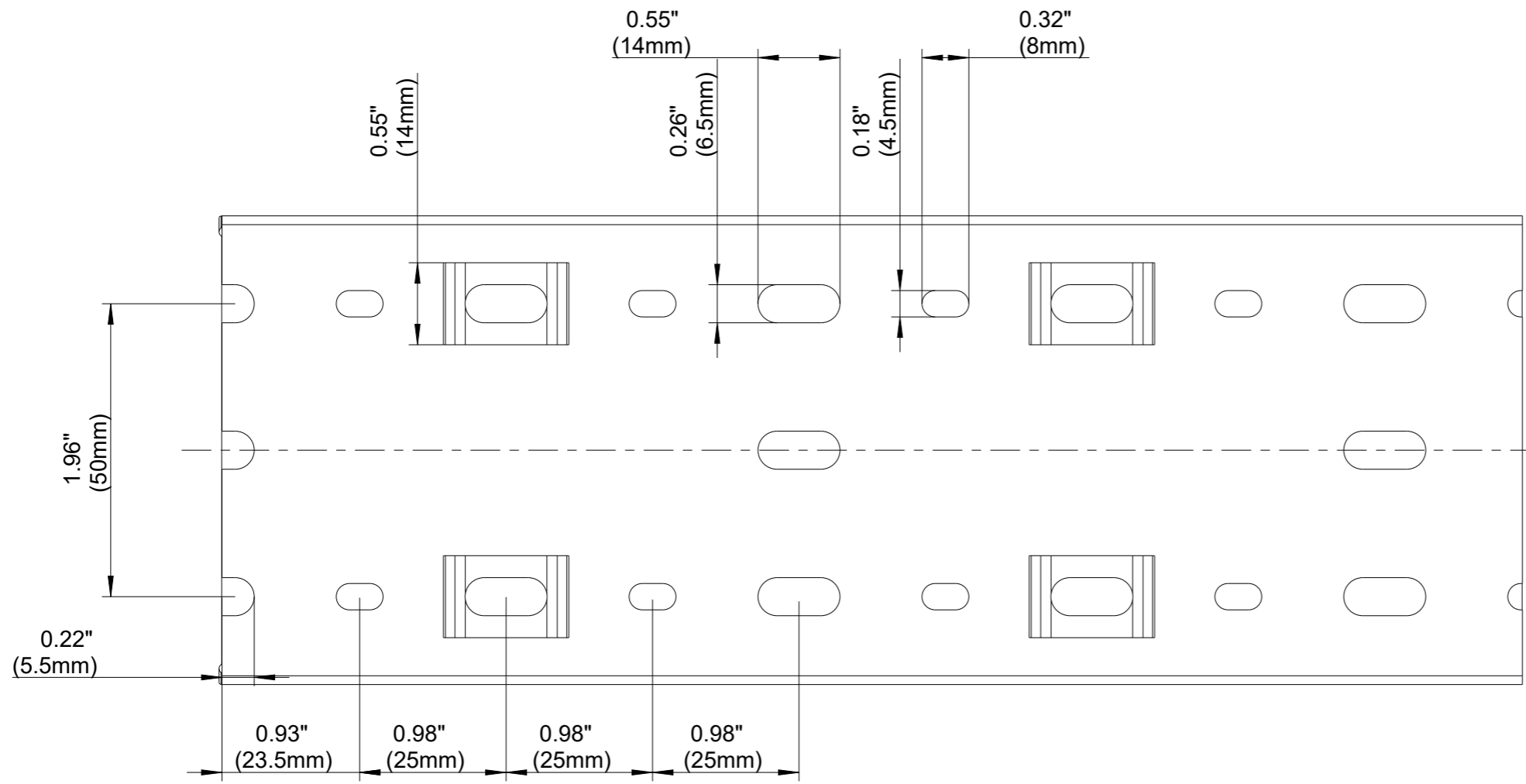
BASE PERFORATION
