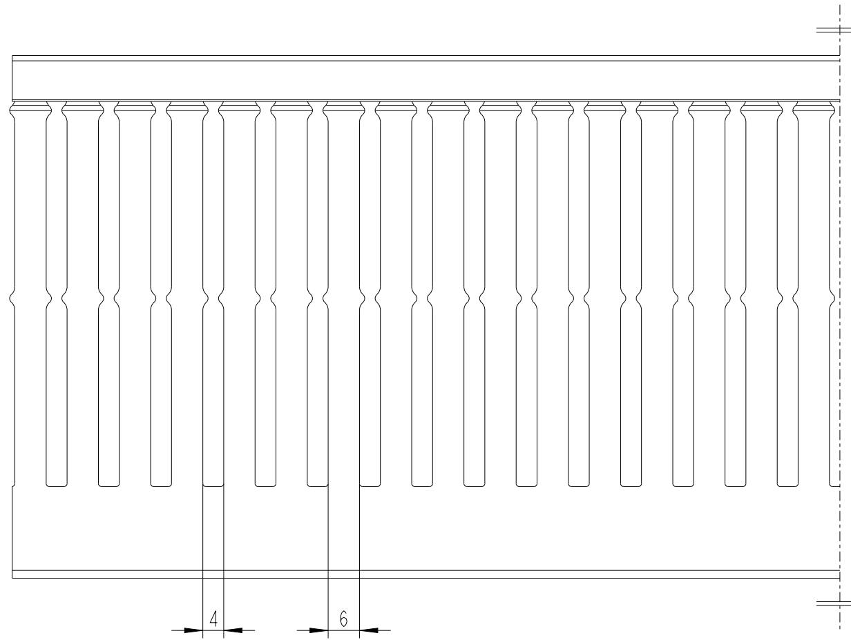
SIDE SECTION
