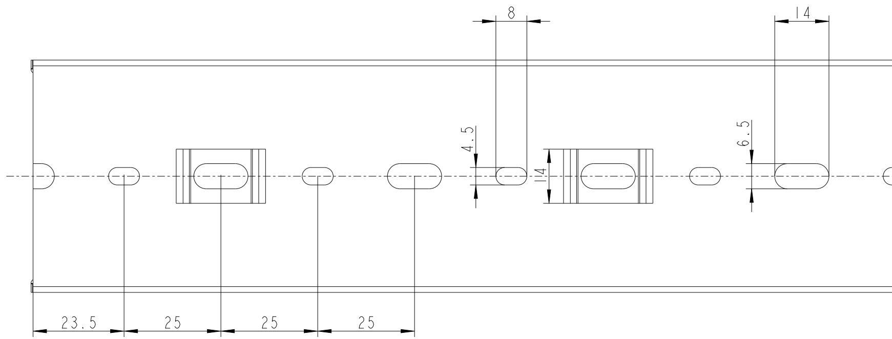
BASE PERFORATION
