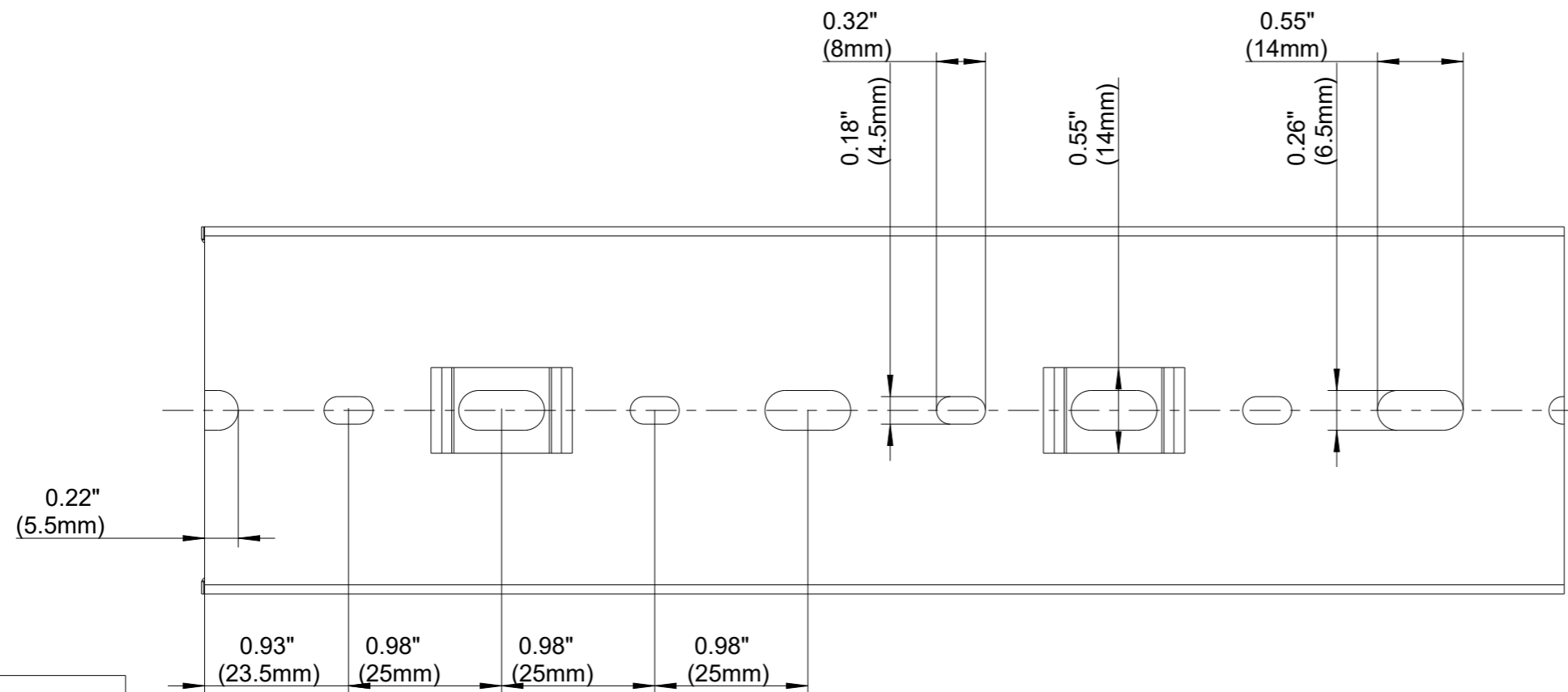
BASE PERFORATION
