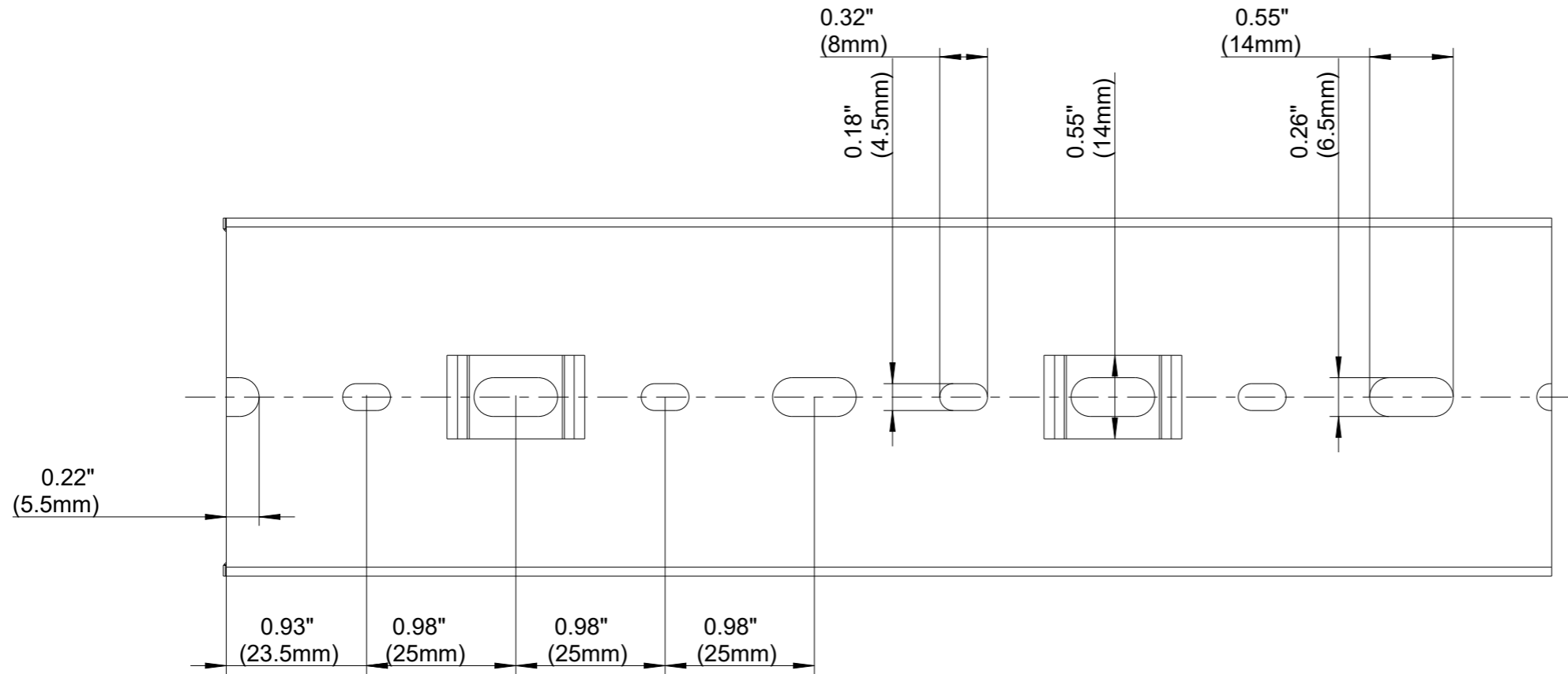
BASE PERFORATION
