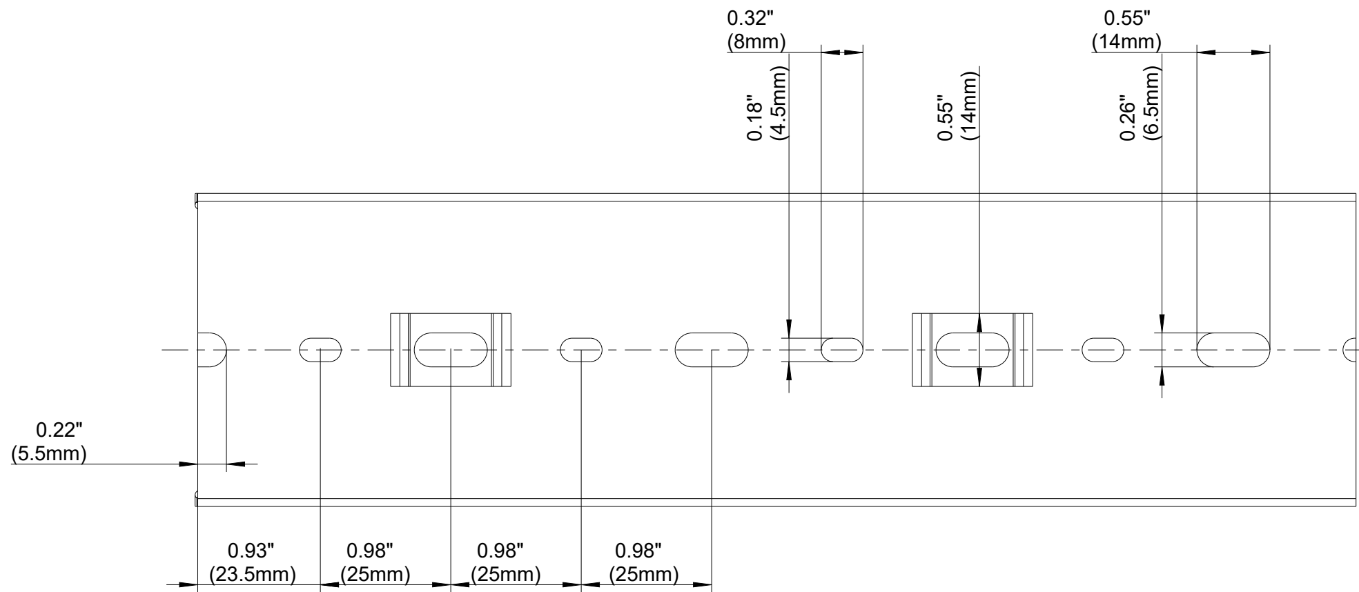
BASE PERFORATION
