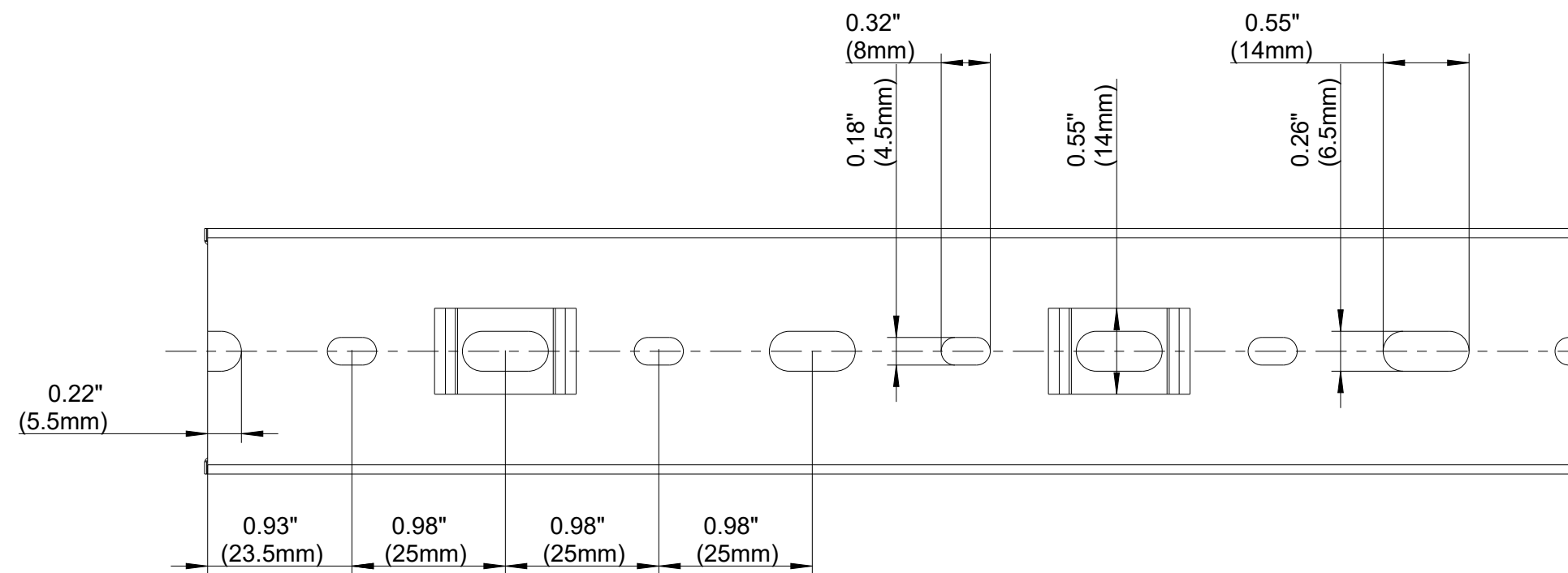
SIDE SECTION
