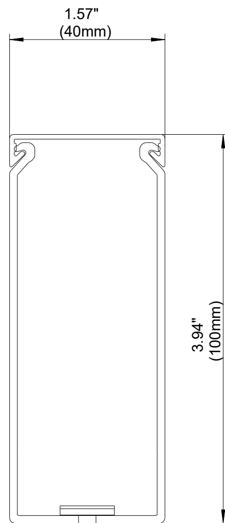
FRONT SECTION
