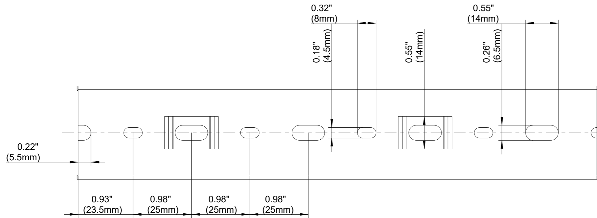
BASE PERFORATION
