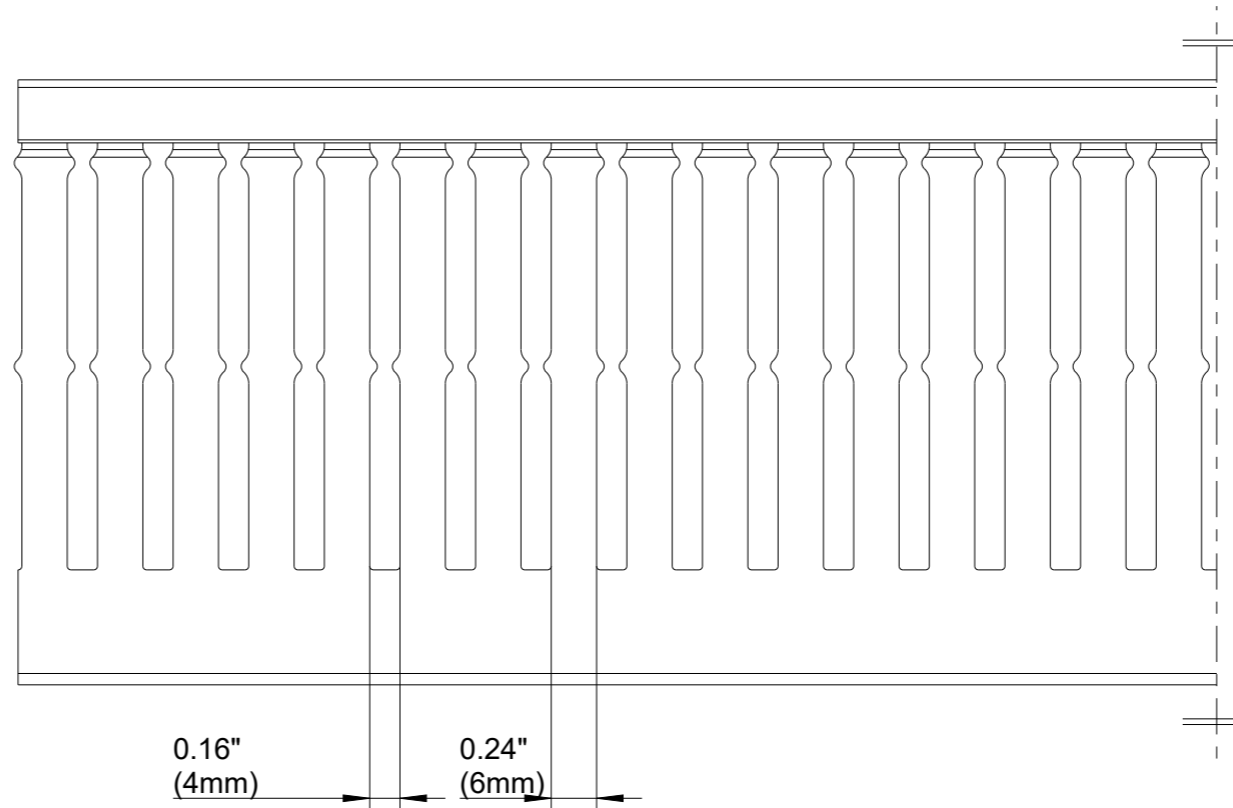
SIDE SECTION
