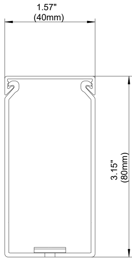
FRONT SECTION
