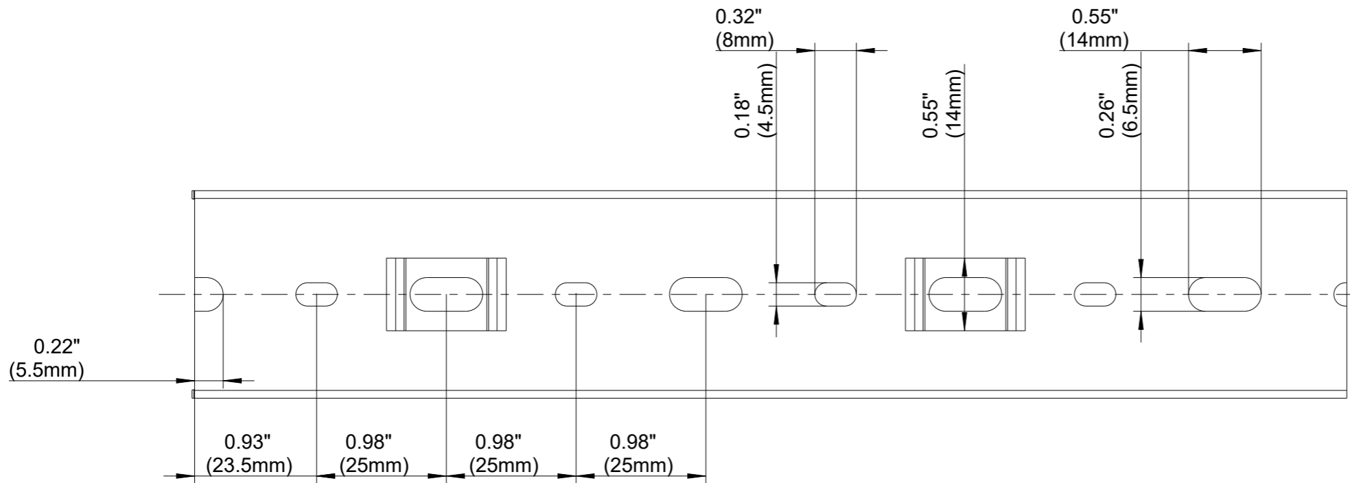
BASE PERFORATION
