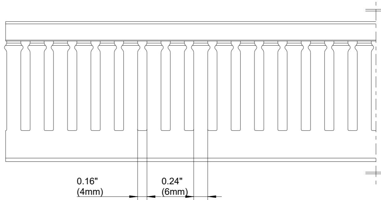
SIDE SECTION
