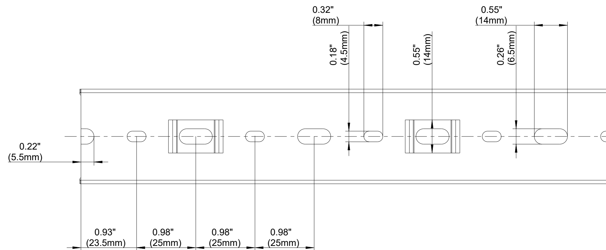
BASE PERFORATION
