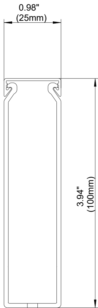
FRONT SECTION
