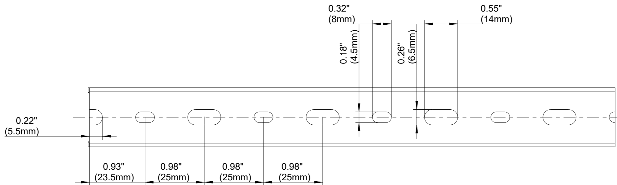
BASE PERFORATION
