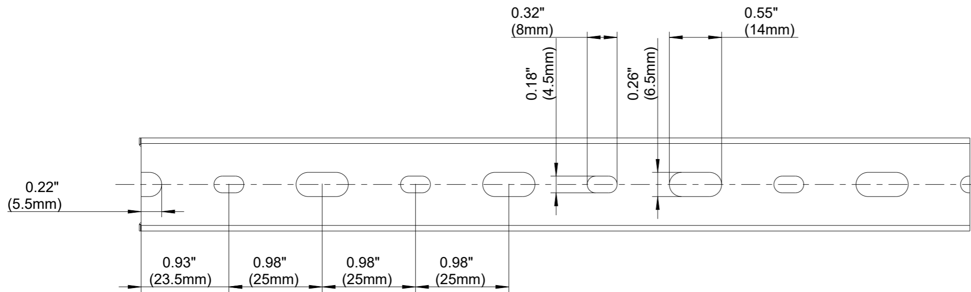
BASE PERFORATION
