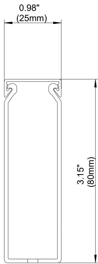
FRONT SECTION
