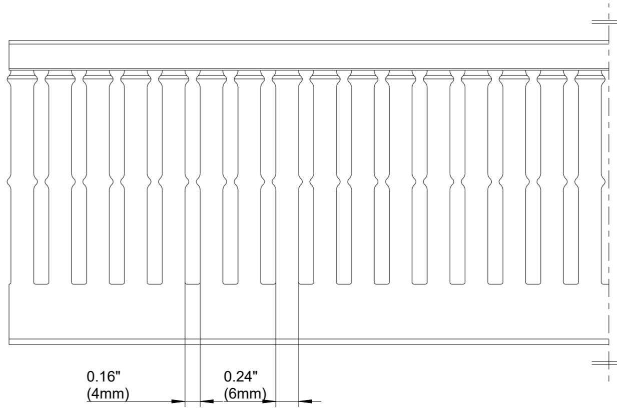
SIDE SECTION
