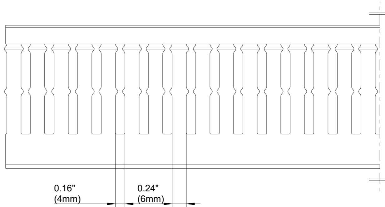
SIDE SECTION
