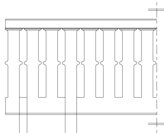
SCALE 1:2 SIDE SECTION
