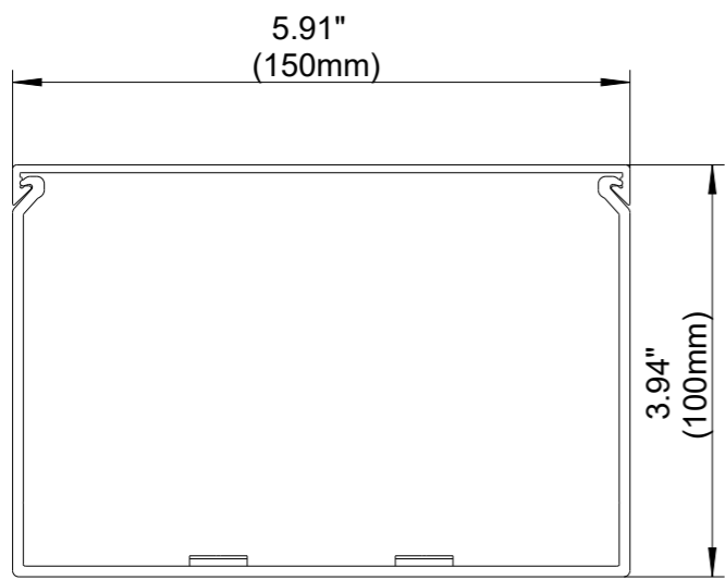
SCALE 1:2 FRONT SECTION
