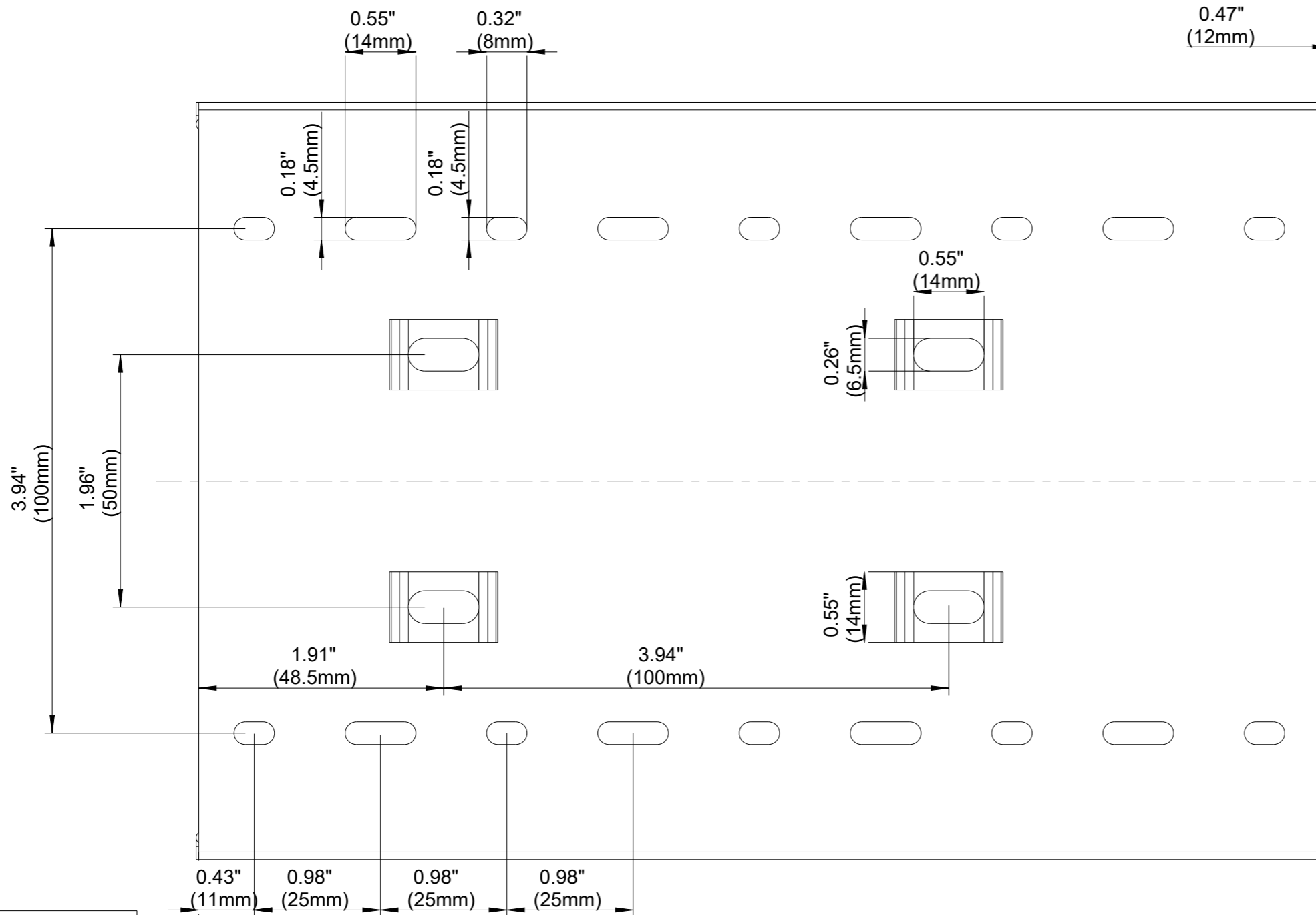
BASE PERFORATION
