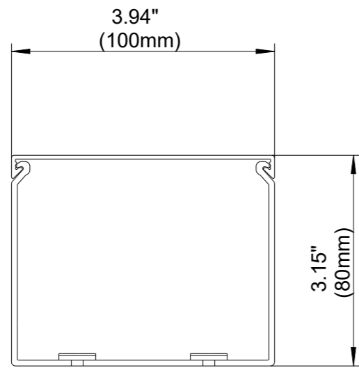
SCALE 1:2 FRONT SECTION
