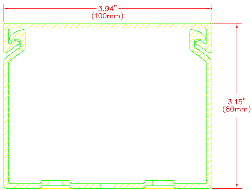
FRONT SECTION
