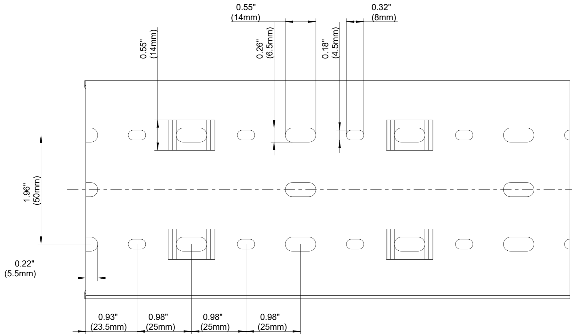
BASE PERFORATION
