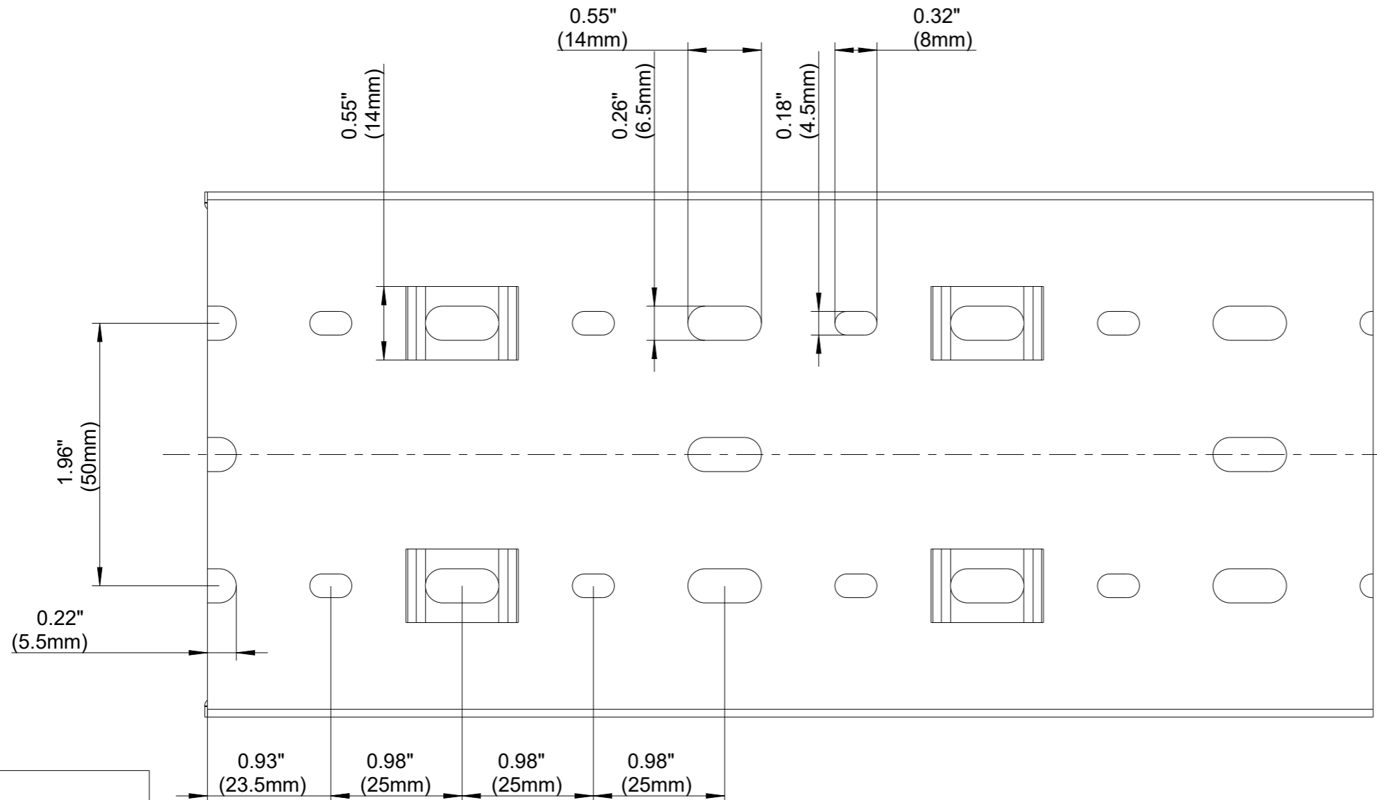
BASE PERFORATION
