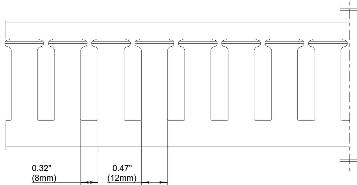
SIDE SECTION
