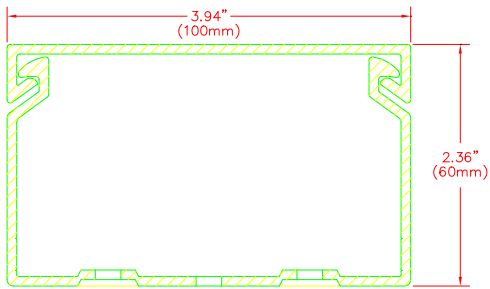
FRONT SECTION
