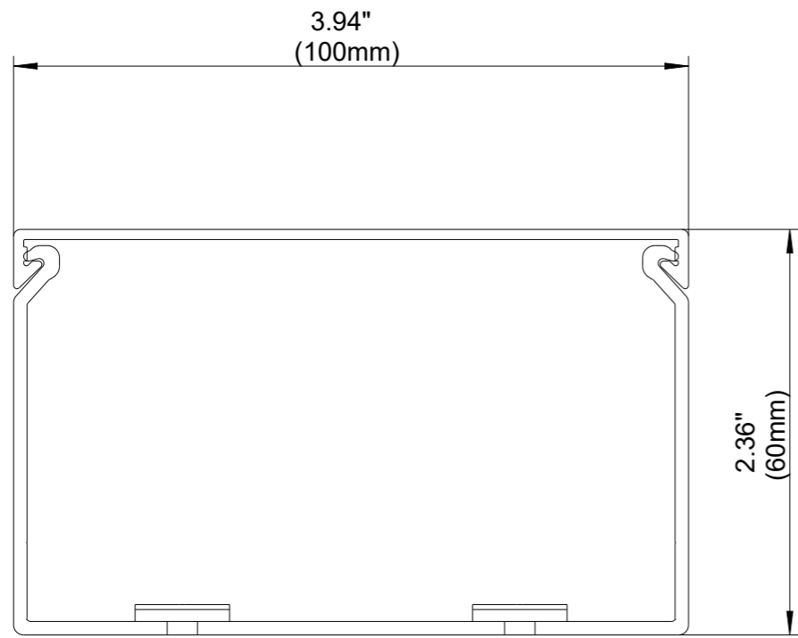
FRONT SECTION
