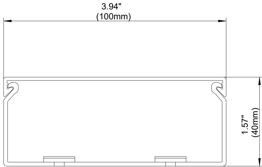
FRONT SECTION
