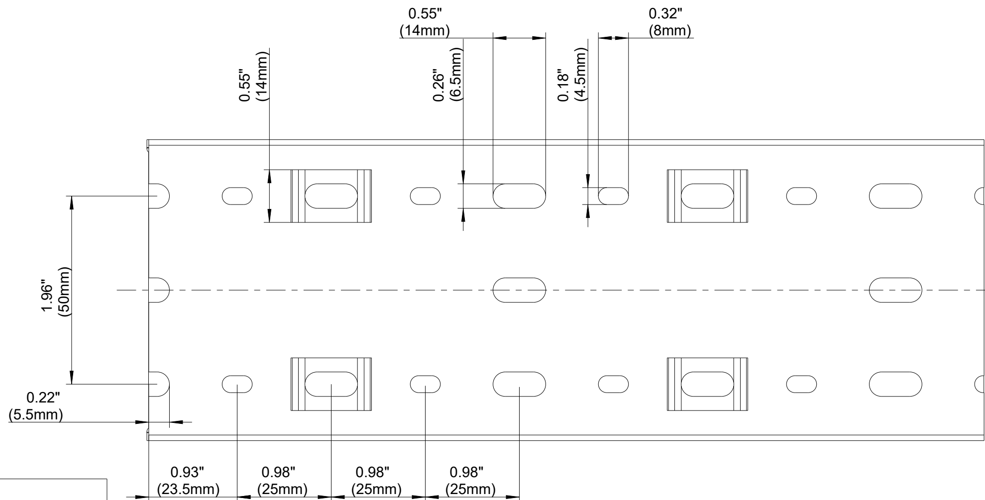
BASE PERFORATION
