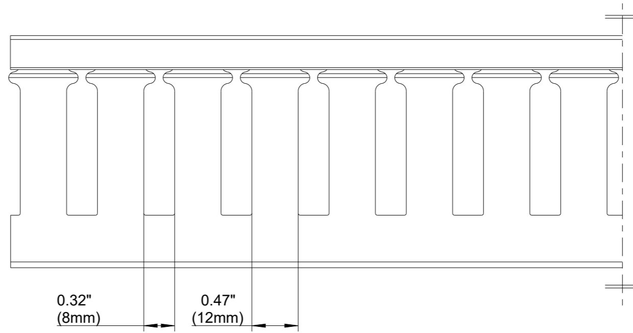
SIDE SECTION
