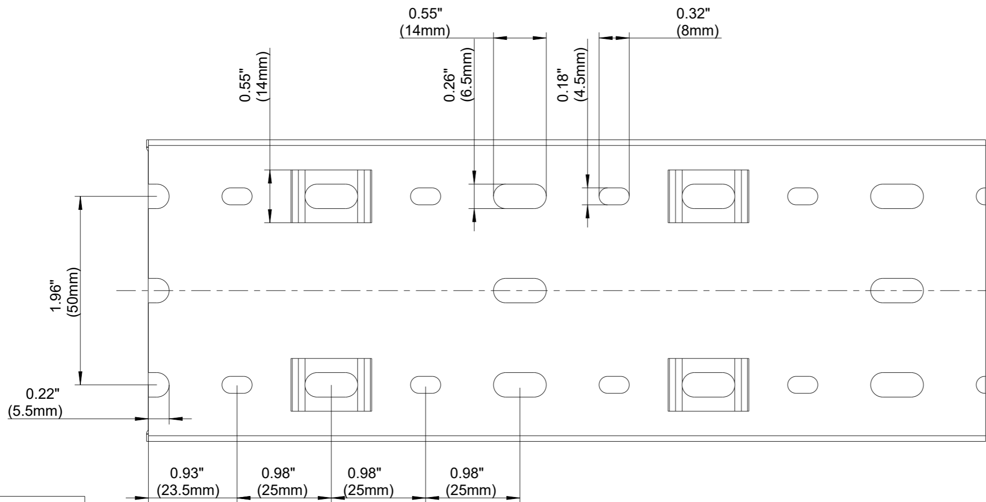
BASE PERFORATION
