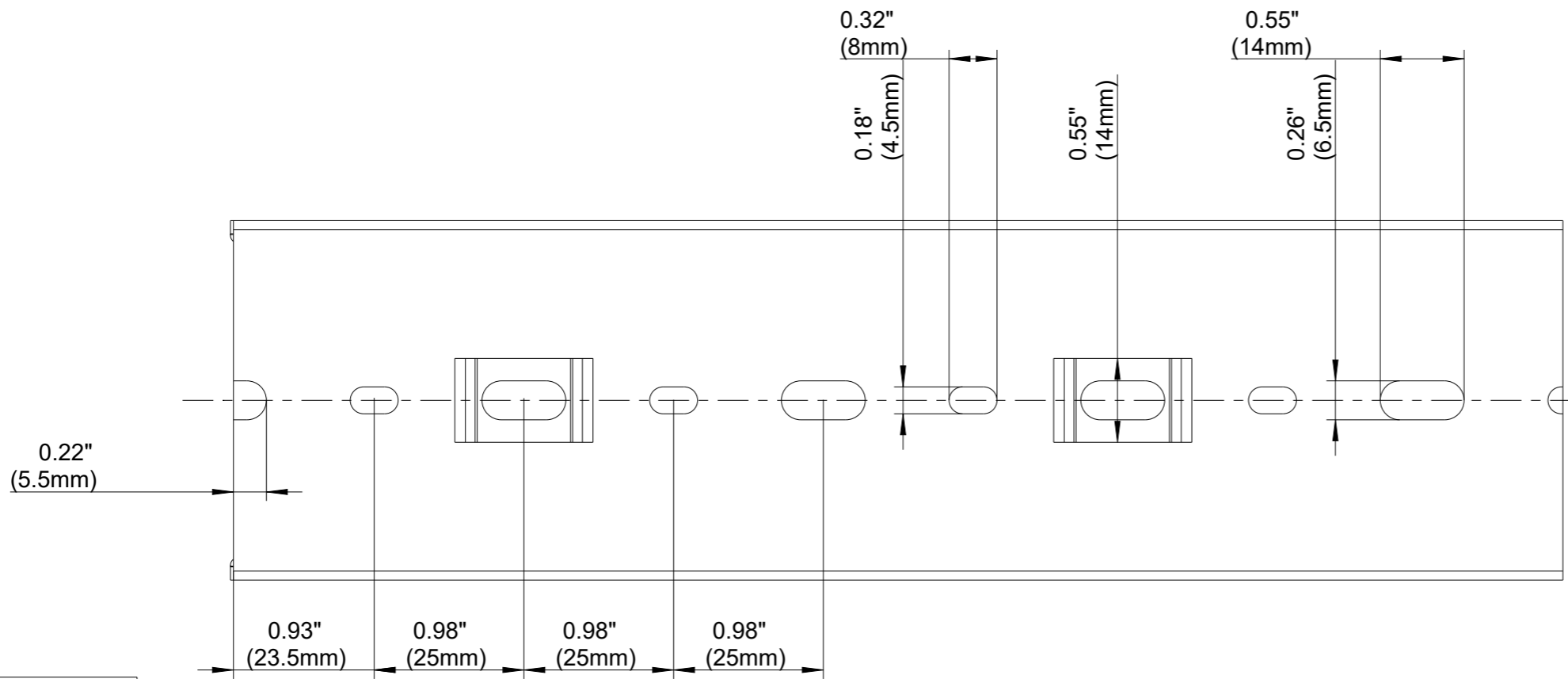
BASE PERFORATION
