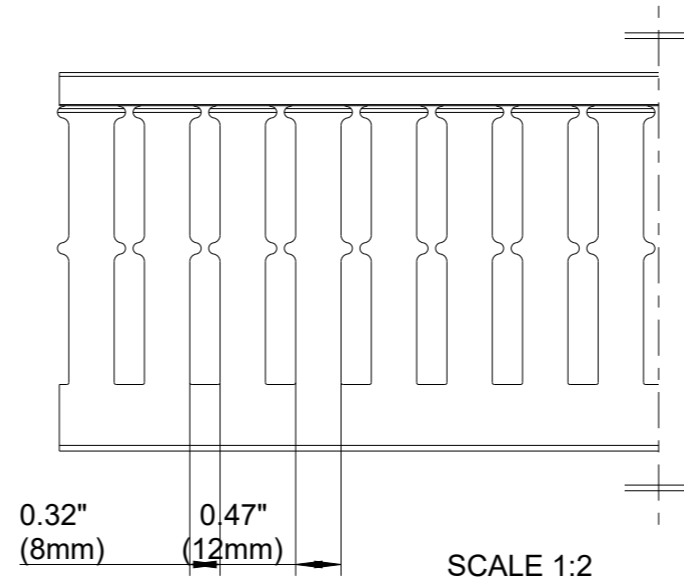
SCALE 1:2 SIDE SECTION
