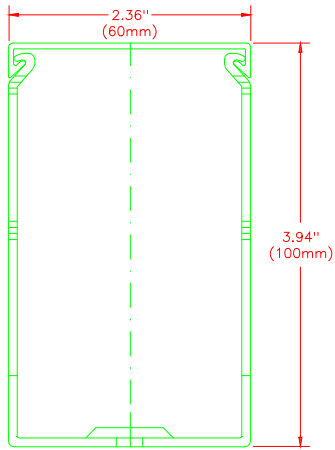
FRONT SECTION
