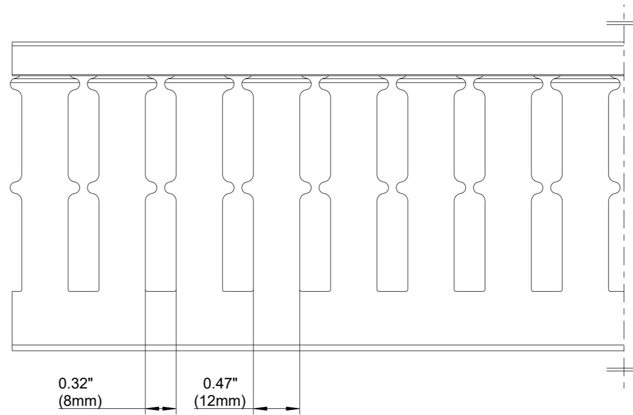
SIDE SECTION
