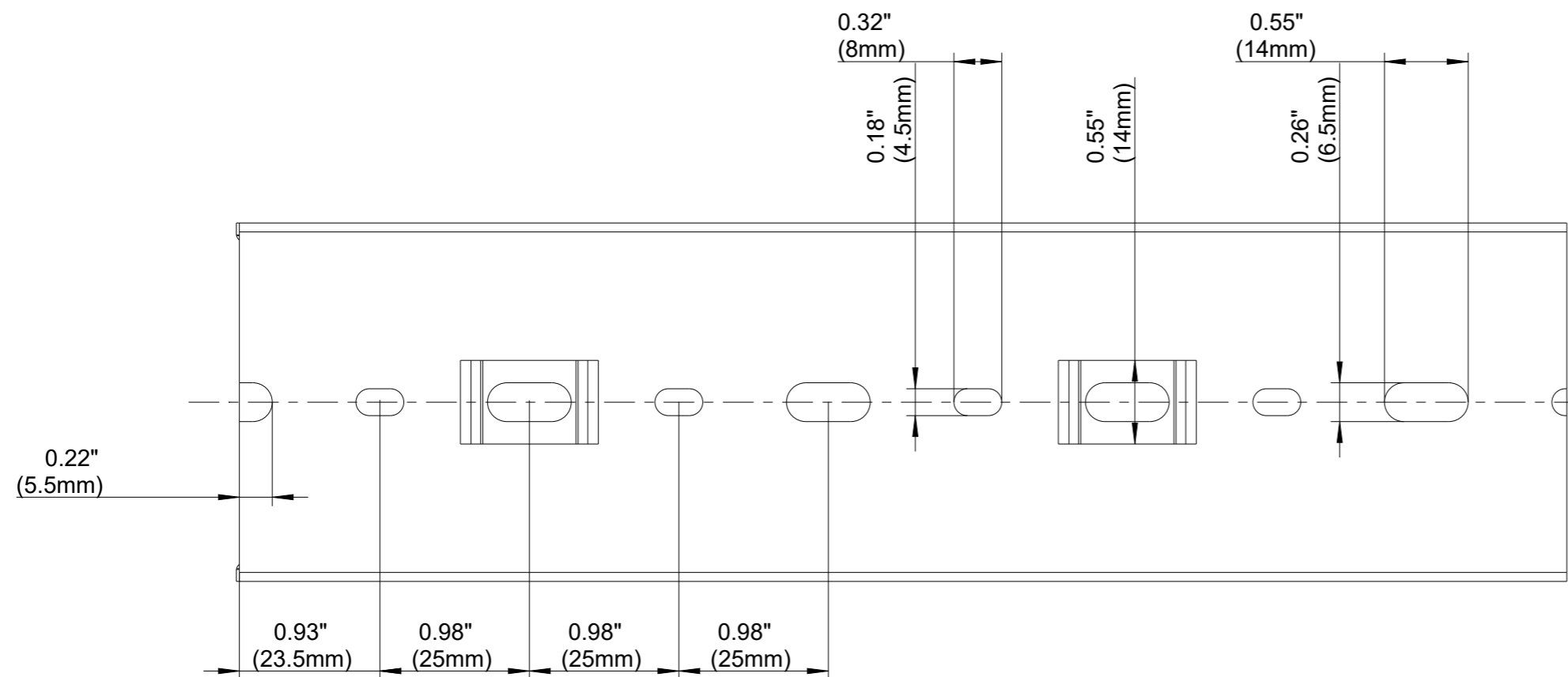
BASE PERFORATION
