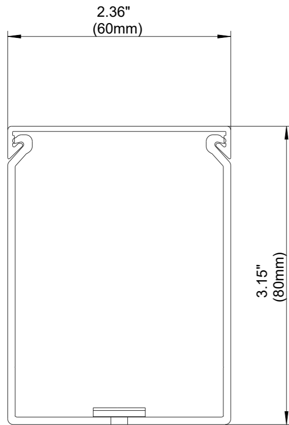
FRONT SECTION
