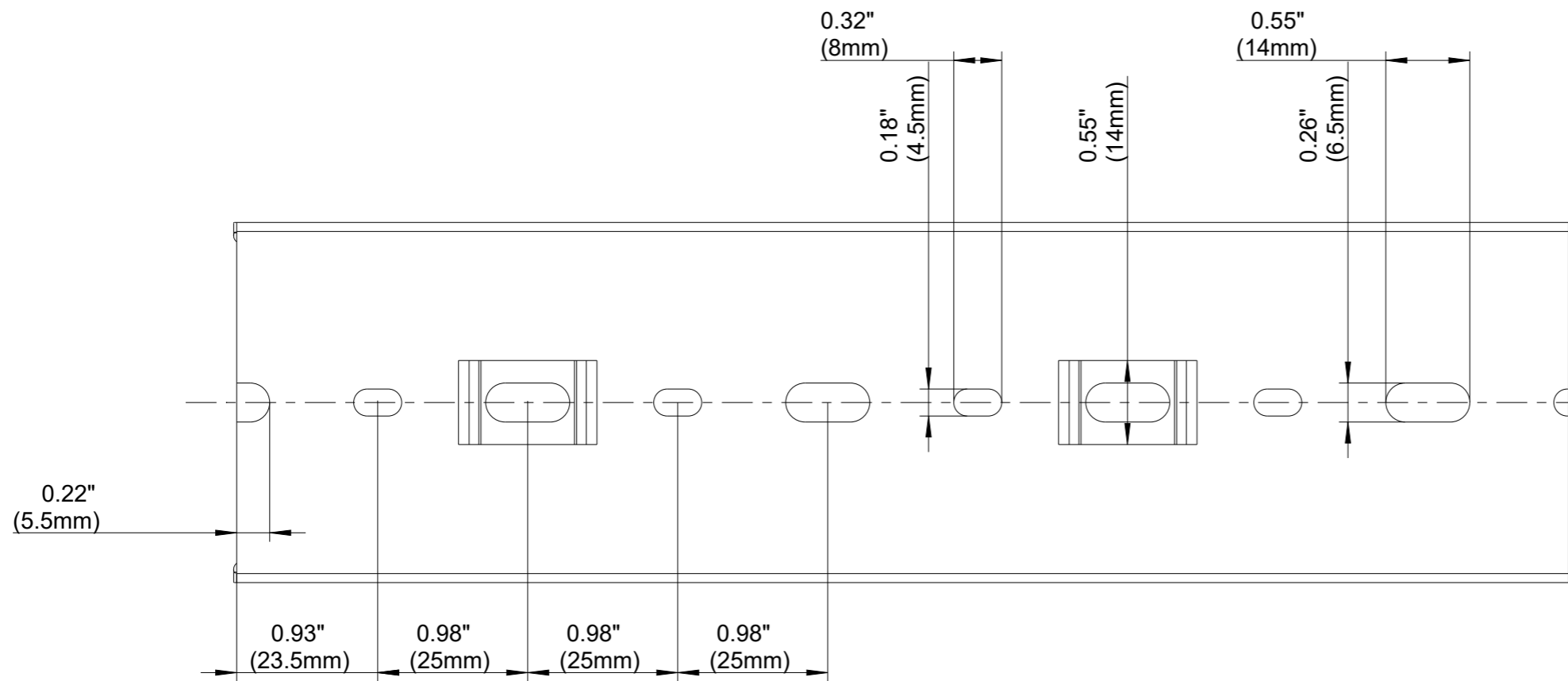
BASE PERFORATION
