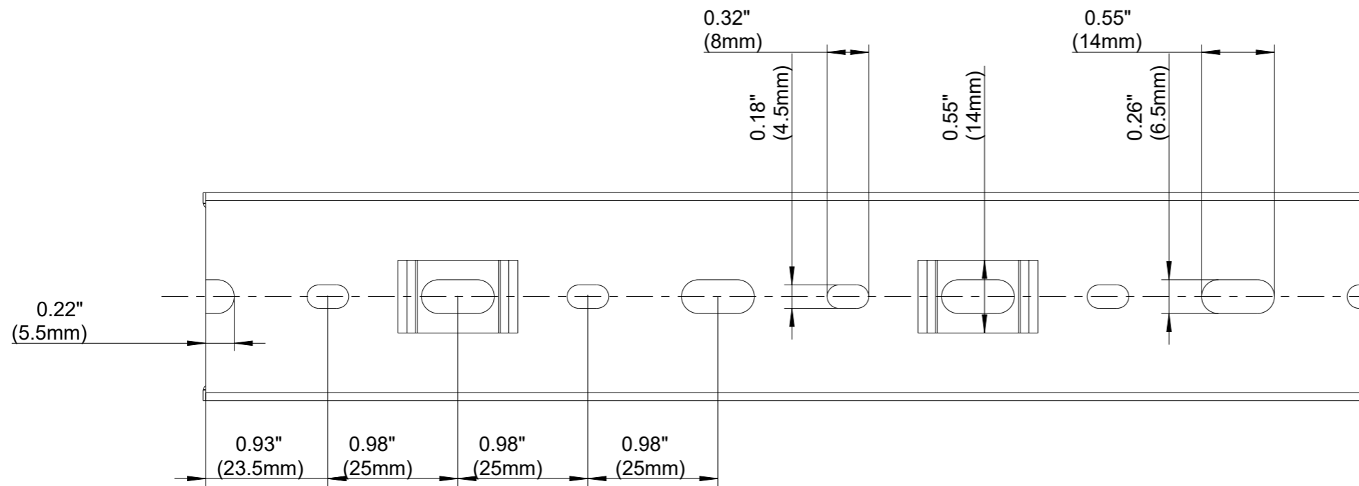
BASE PERFORATION
