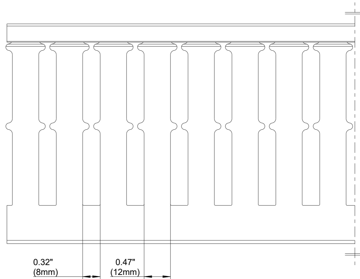
SIDE SECTION
