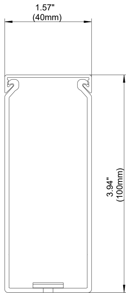
FRONT SECTION
