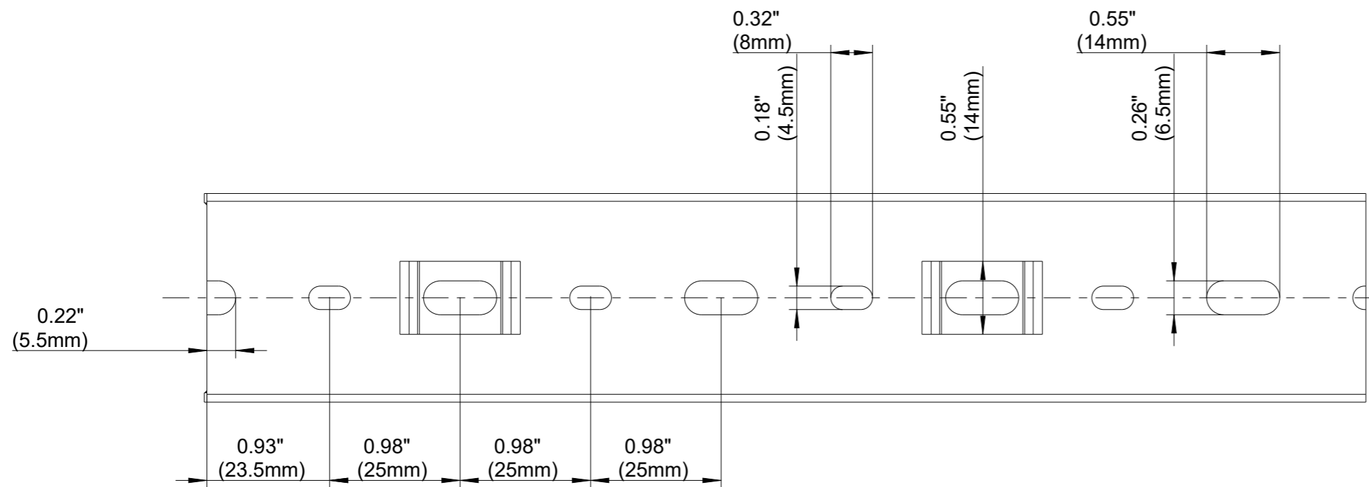
BASE PERFORATION
