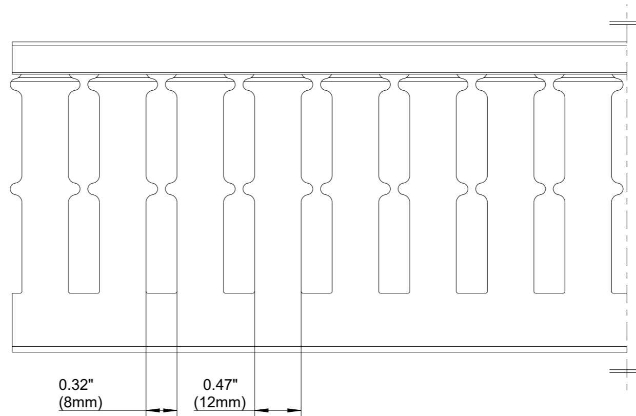
SIDE SECTION
