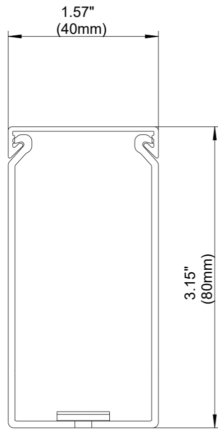
FRONT SECTION
