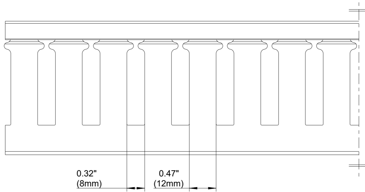
SIDE SECTION
