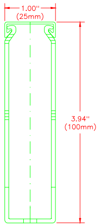
FRONT SECTION
