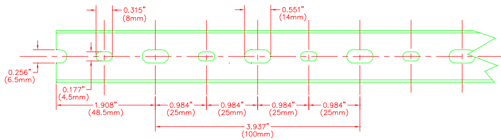
BASE PERFORATION
