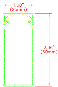
FRONT SECTION
