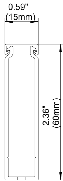
FRONT SECTION
