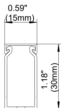
FRONT SECTION
