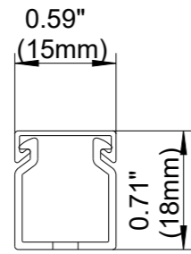
FRONT SECTION
