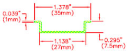
FRONT SECTION
