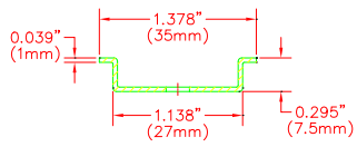
FRONT SECTION
