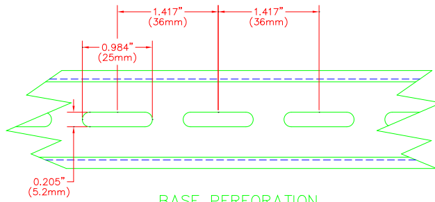
BASE PERFORATION
