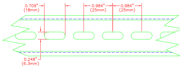
BASE PERFORATION
