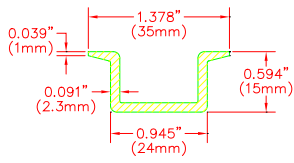
FRONT SECTION
