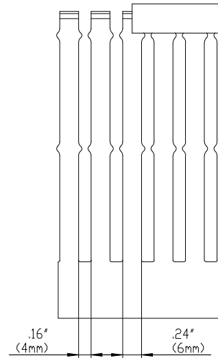
SIDE SECTION
