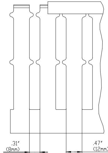
SIDE SECTION
