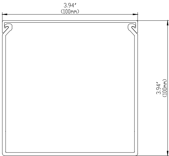
FRONT SECTION
