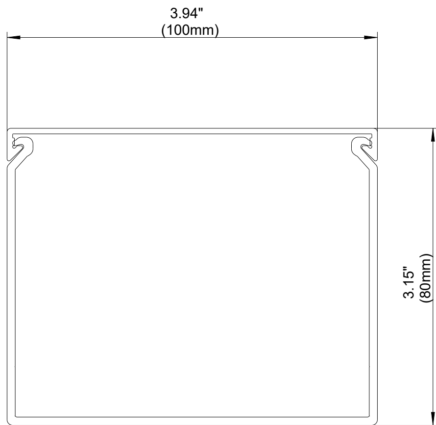
FRONT SECTION
