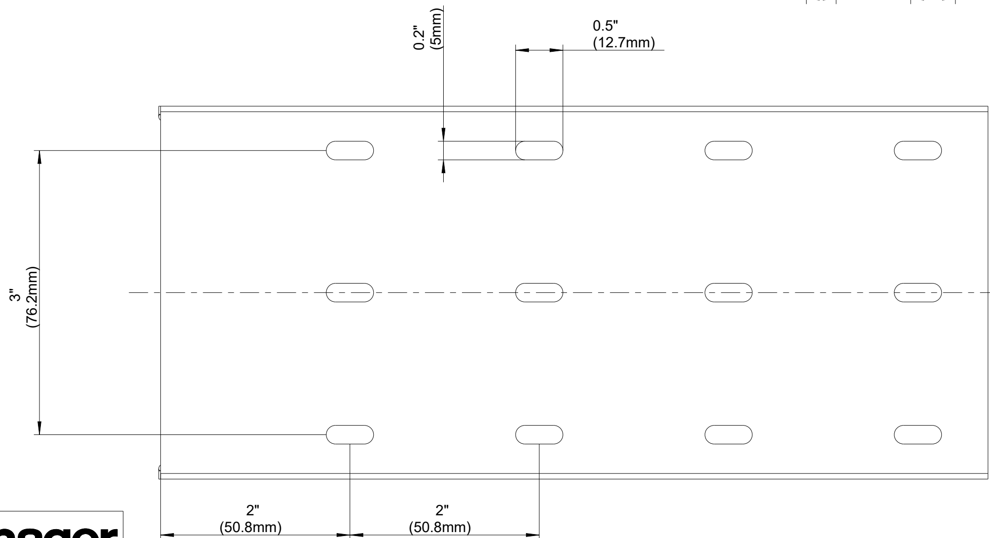
BASE PERFORATION
