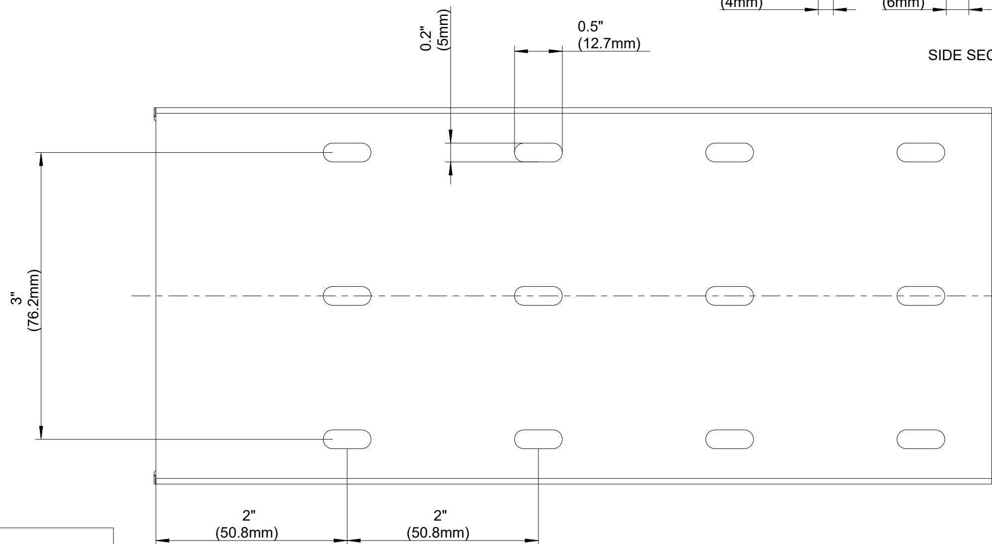
BASE PERFORATION
